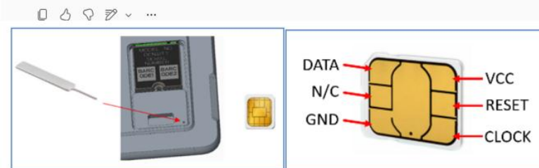
Figure 3. Nano SIM card slot
